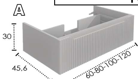
FORTUNA 30 1 CAJÓN/DRAWER/TIROIR - PLAN NON INCLUS/WITHOUT WORKTOP
